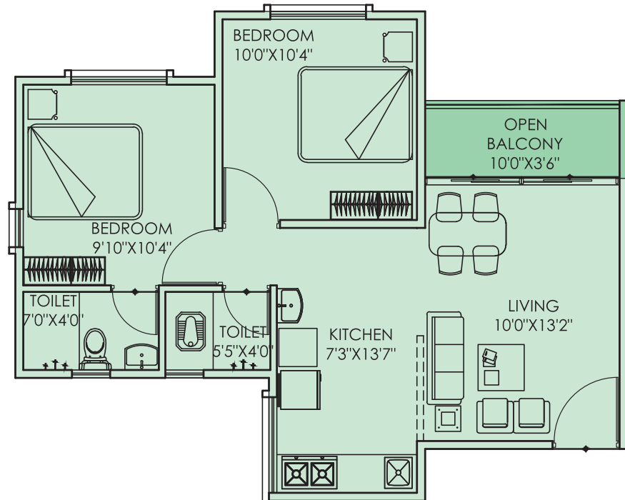
2 BHK TYPE- BIG RERA CARPET AREA= 555 SQ.FT. FLAT NO. SERIES- 2,3
