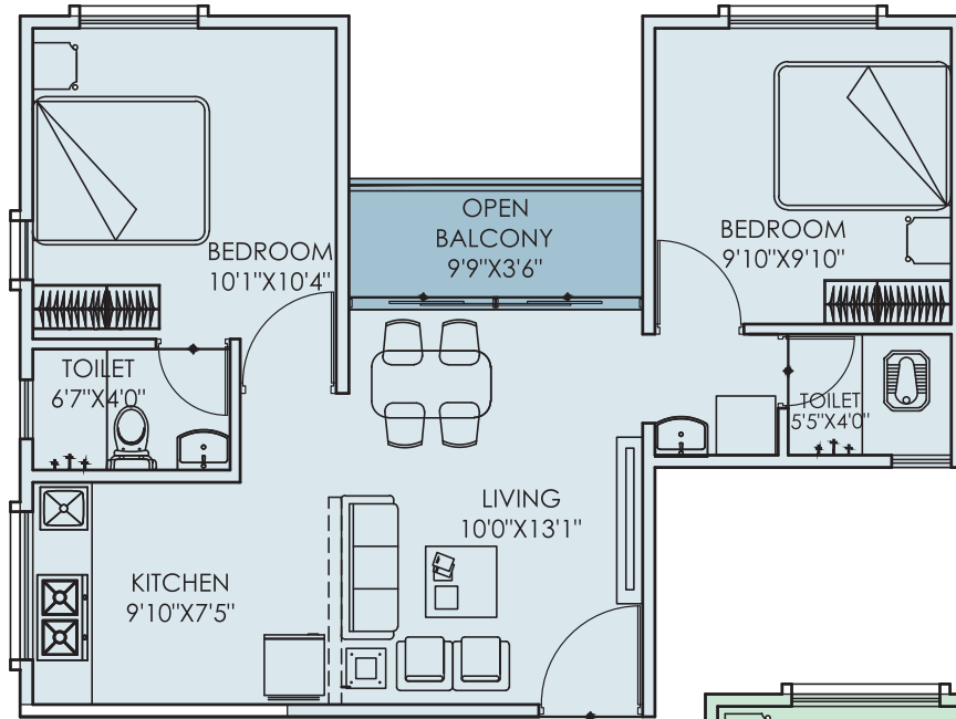
2 BHK TYPE- SMALL RERA CARPET AREA= 542 SQ.FT. FLAT NO. SERIES- 10,11
